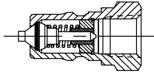
Nipple
