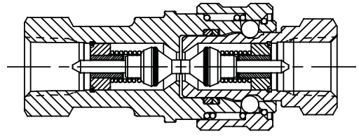
Coupling
