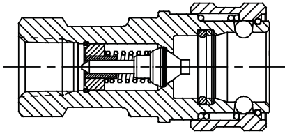
Coupler
