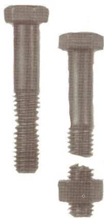
STRETCHING and BREAKING
